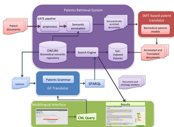
Figure 1: General architecture of the multilingual retrieval system
