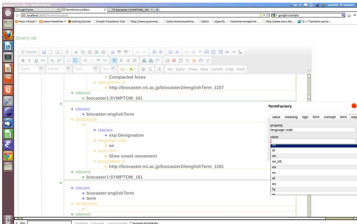
Figure 1. Editing TF/XHTML with a textarea editor
